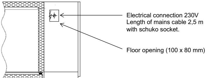
Picture 4: Plan view refrigerated counter (for connecting to a central cooling system)
